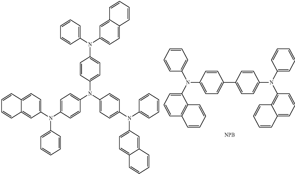
2-TNATA
